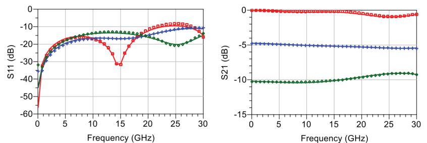
Model vs. Measured Series 2-port S-parameter Data - ATT-SINT-TT9-001 Modelithics Model for TT9 SMT Attenuator Series 3 Attenuator Values on 6.6 mil Rogers 4350B (H/Er = 1.7 mil)
